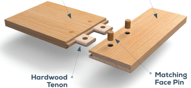
Solid Two-Piece Mortised Rail
